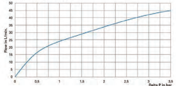
Mixing valves T9107
